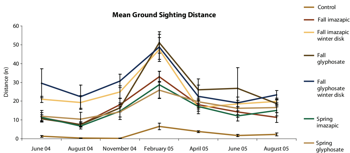
Figure 14. Ground sighting distance is the maximum distance a prone observer can see without being obstructed by vegetation. This measurement is used as an index of mobility for gamebird broods.
