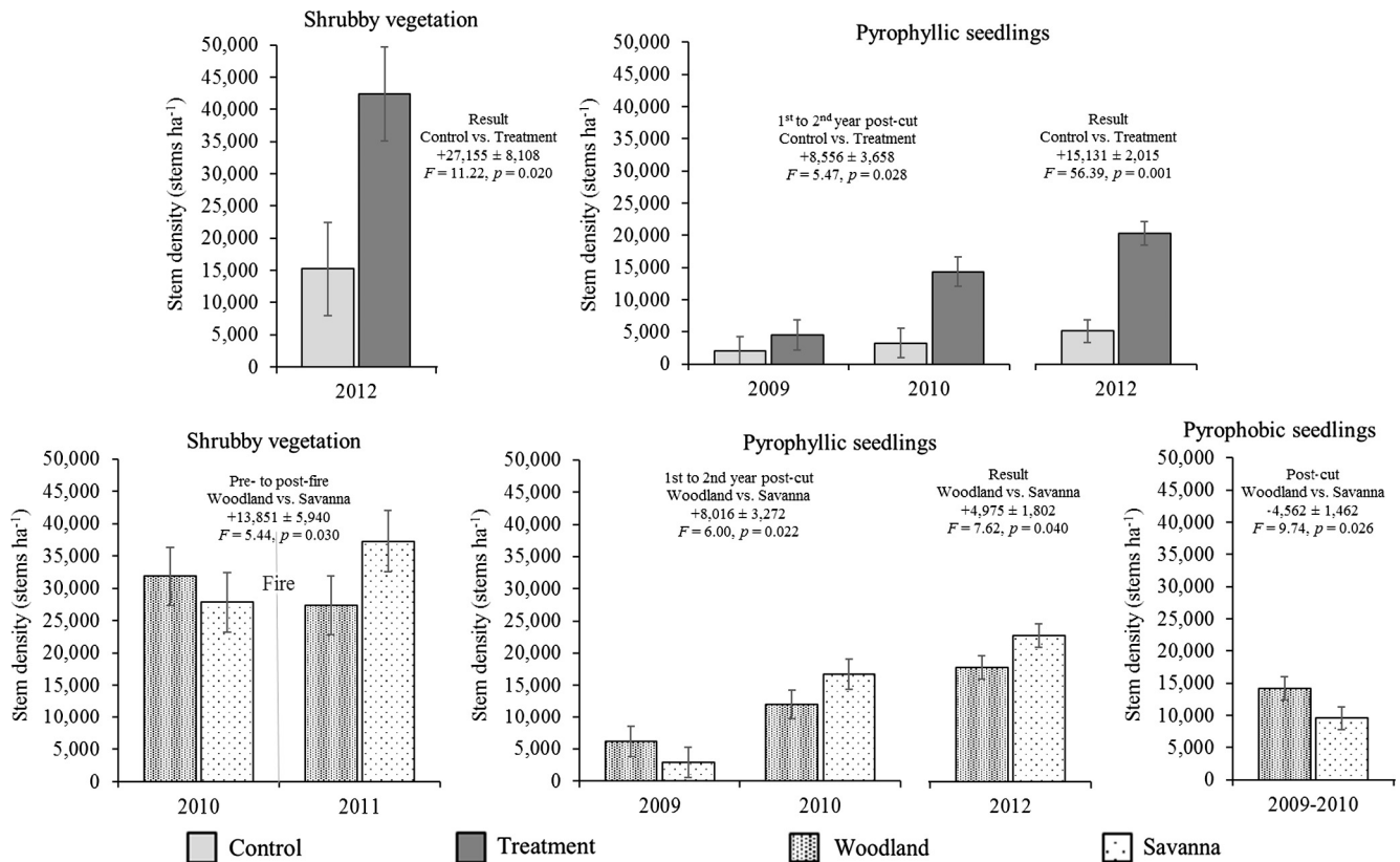
Fig. 2. All significant ( \alpha = 0.05 ) contrasts for shrubby vegetation and seedling stem density (stems \text{ha}^{-1} ) during an oak woodland and savanna restoration experiment (2008–2012) at Catoosa Wildlife Management Area, Cumberland County, TN. Treatment contrasts included Woodland ( 14 \text{ m}^2 \text{ ha}^{-1} residual basal area) vs. Savanna ( 7 \text{ m}^2 \text{ ha}^{-1} residual basal area) post-cut (2009 and 2010), Spring vs. Fall burns post-fire (2011 and 2012), and end result (2012); Control (unmanaged stands) vs. Treatment (all managed stands), Woodland vs. Savanna, and Spring vs. Fall fire. Interaction contrasts included Control vs. Treatment and Woodland vs. Savanna over all year intervals (2008–2012) and Spring vs. Fall fire over post-fire intervals (2010–2012). See Table A1 for species composing each group. Seedlings were \geq 30.5 \text{ cm} but < 1.4 \text{ m} tall.
